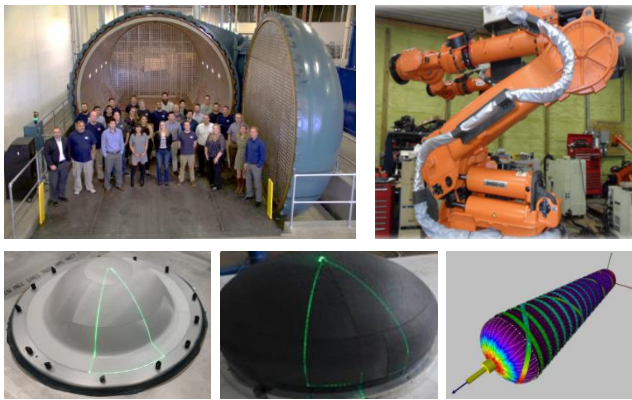
SDC's Manufacturing Facility includes State-of-the-Art Composite Processing and Machining Capabilities
