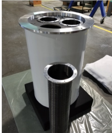
PEI Mock-up of "Mini-MAC" concept with continuous outer Copyright 2018 Pacific Engineering, Inc
